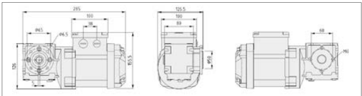
Connection dimensions for Motors AC D16-120W
