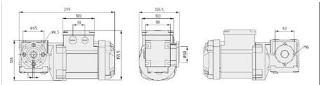
Connection dimensions for Motors AC D16-180W
