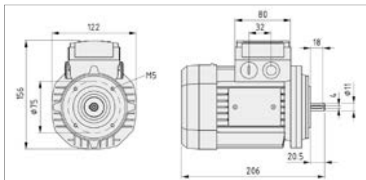
Connection dimensions for Motors AC D11
